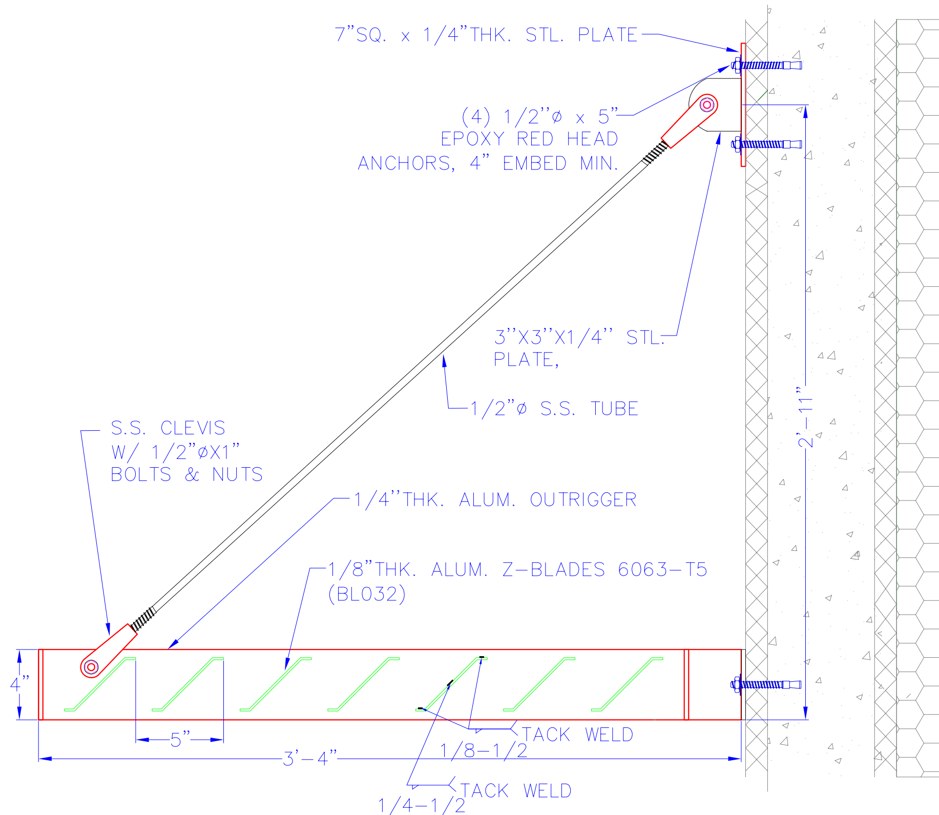
CANOPY SECTION (@ MASONRY WALL)
