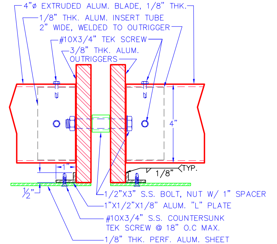
(a) ALUM. OUTRIGGERS - SECTION DETAIL
