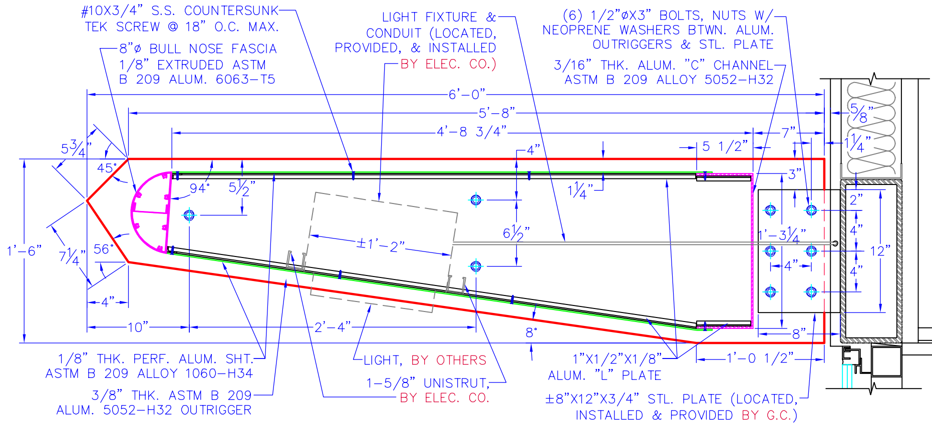
EXTERIOR CANOPIES - SECTION
