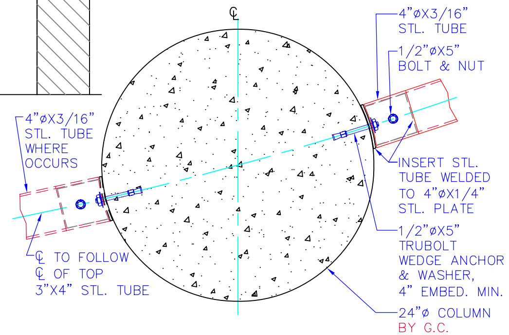
⑩ 4"Ø STL. TUBE ATTACH. DETAIL
