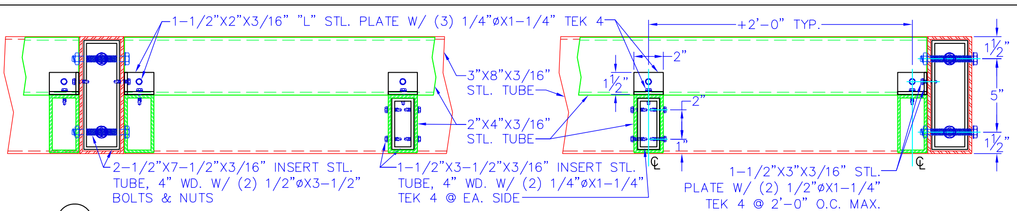
⑨ PATIO SECTION DETAIL
