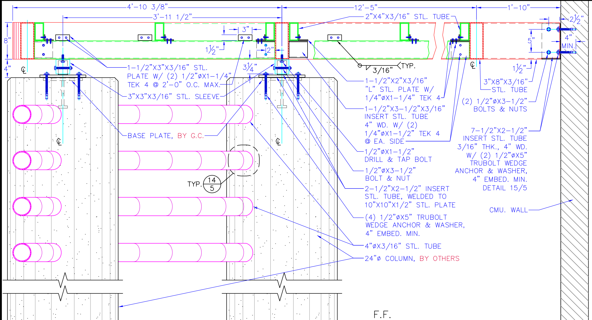
⑧ PATIO SECTION
