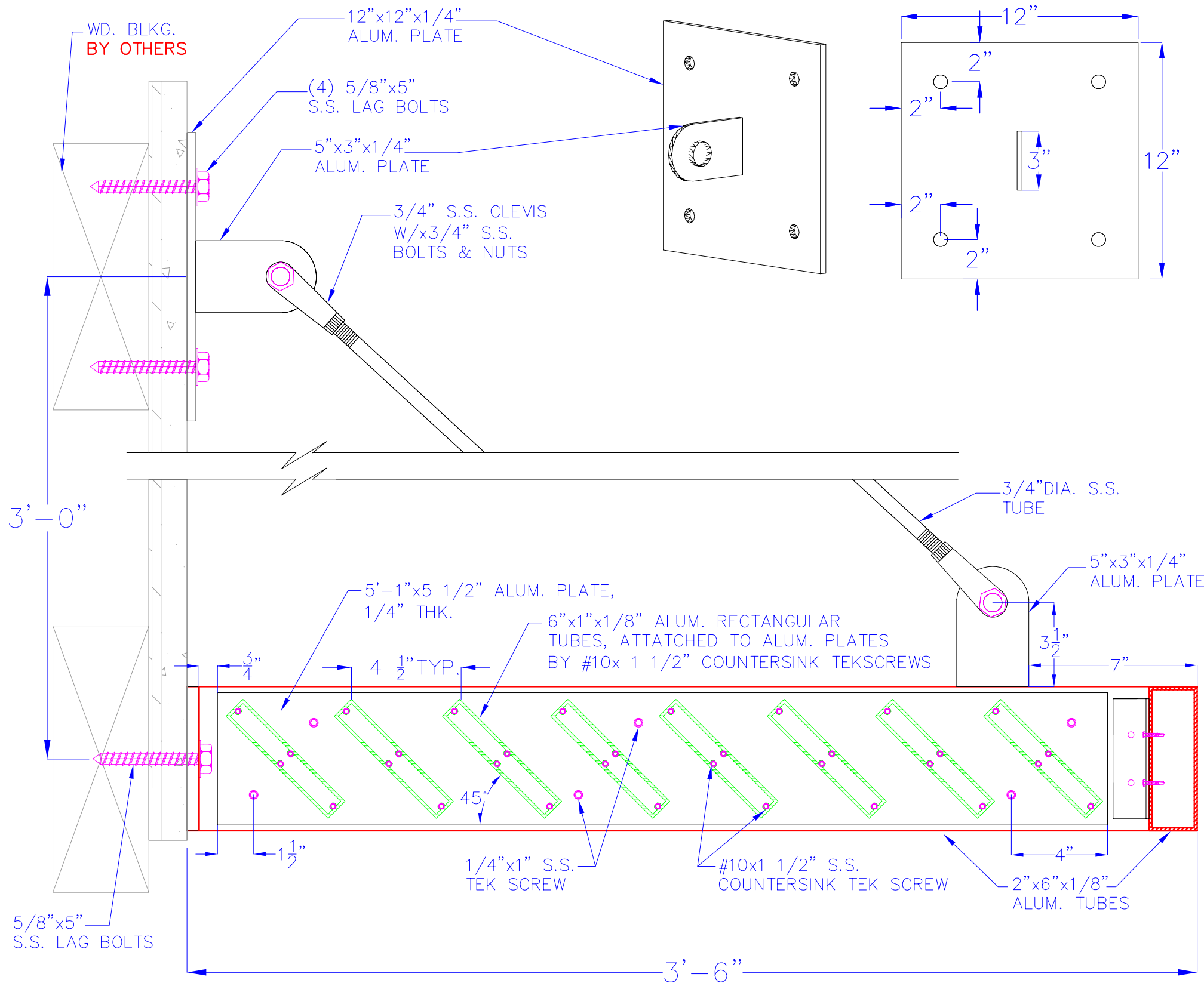
SUNSHADE SECTION
